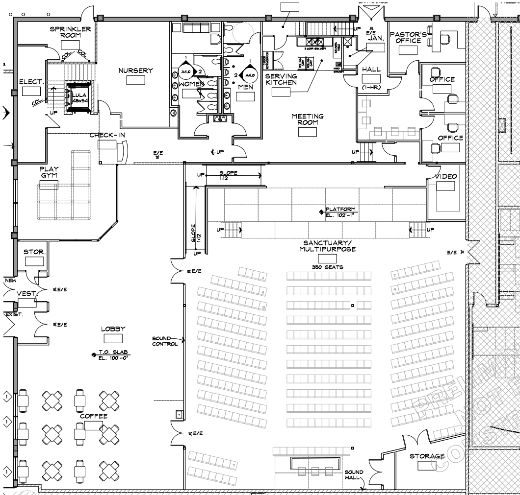
CANVAS CHURCH - FIRST FLOOR
