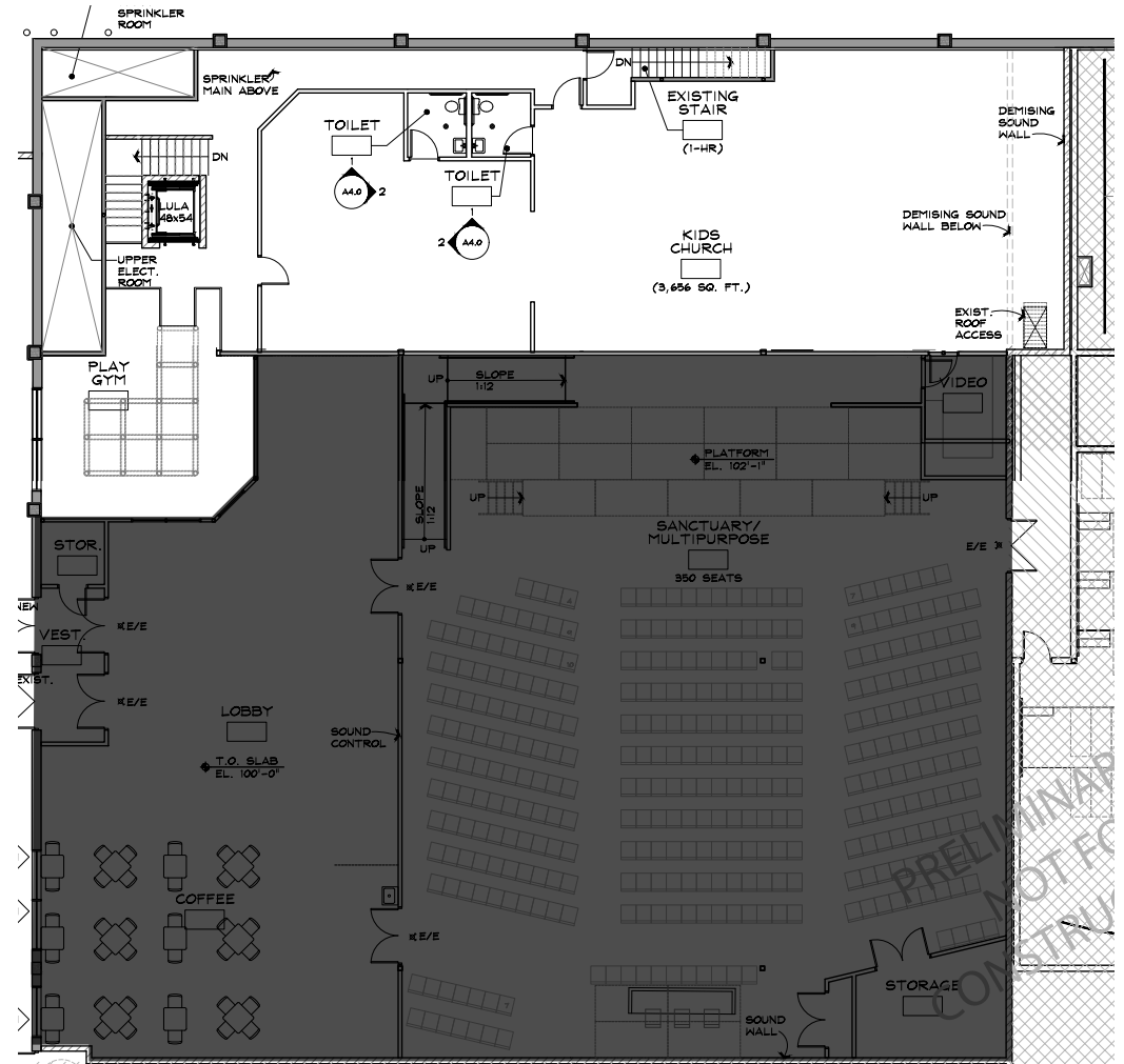
CANVAS CHURCH - SECOND FLOOR
